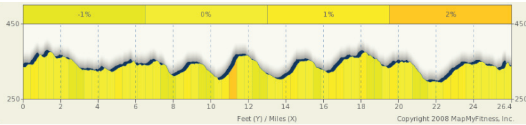
Elevation Chart
